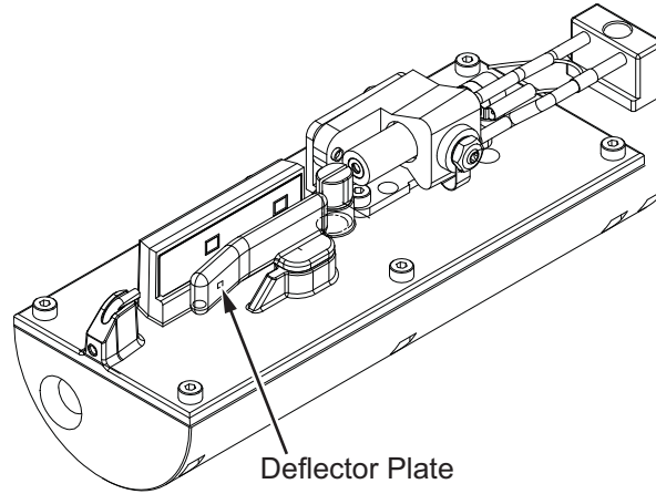
Figure 6-6: Clean the Deflector Plate (Videjet 1650)
