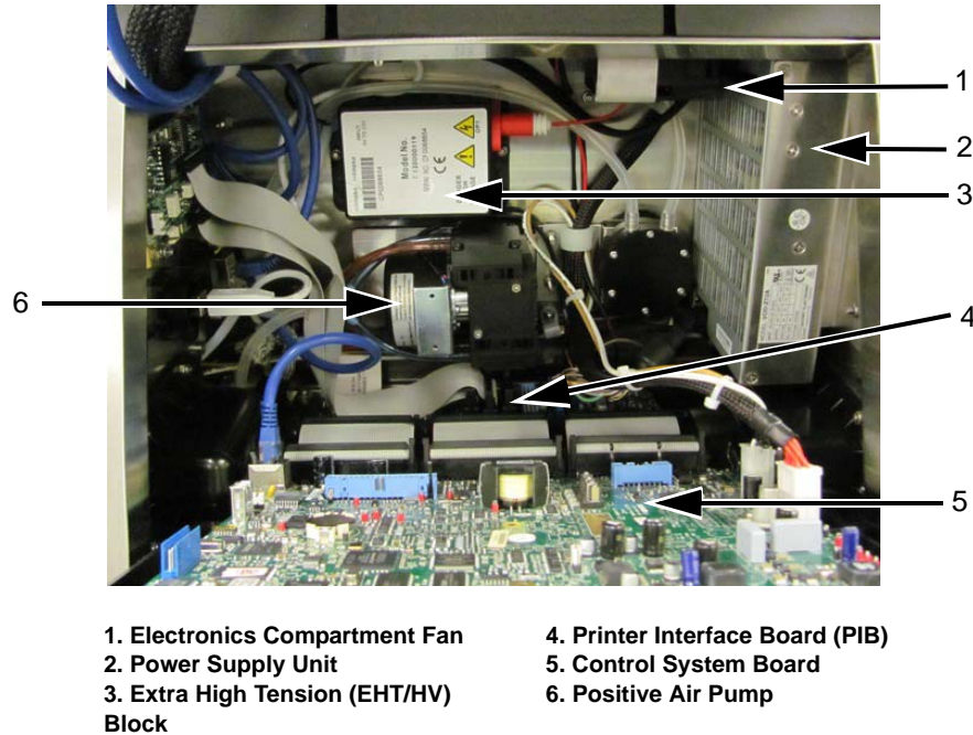
Figure 3-4: Electronics Compartment
