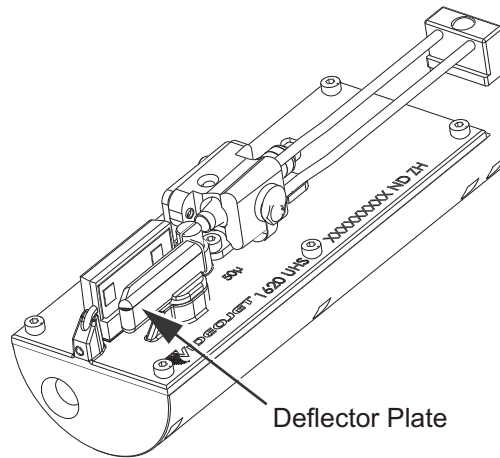
Figure 6-7: Clean the Deflector Plate (Videjet 1650 UHS - 50 Micron)
